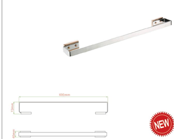
Model: JQS-V009 单杆 Single towel rod
