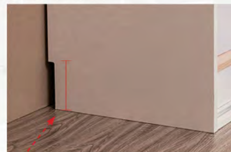
Baseboard,normal size:20mm*120mmH
